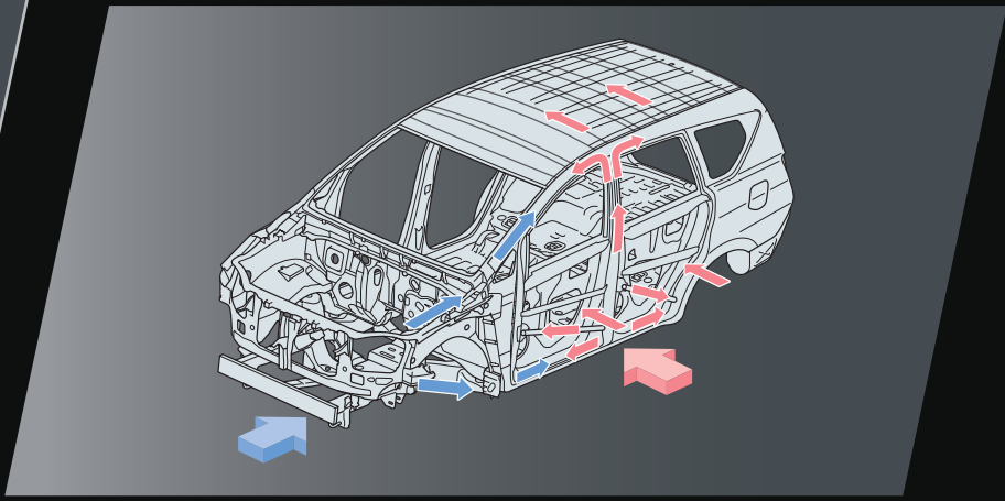
GOA Body | High strength body structure that effectively absorbs impacts and distributes it evenly during unforeseen collisions, thereby reducing passenger and pedestrian injuries
