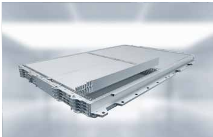
BYD Blade Battery
