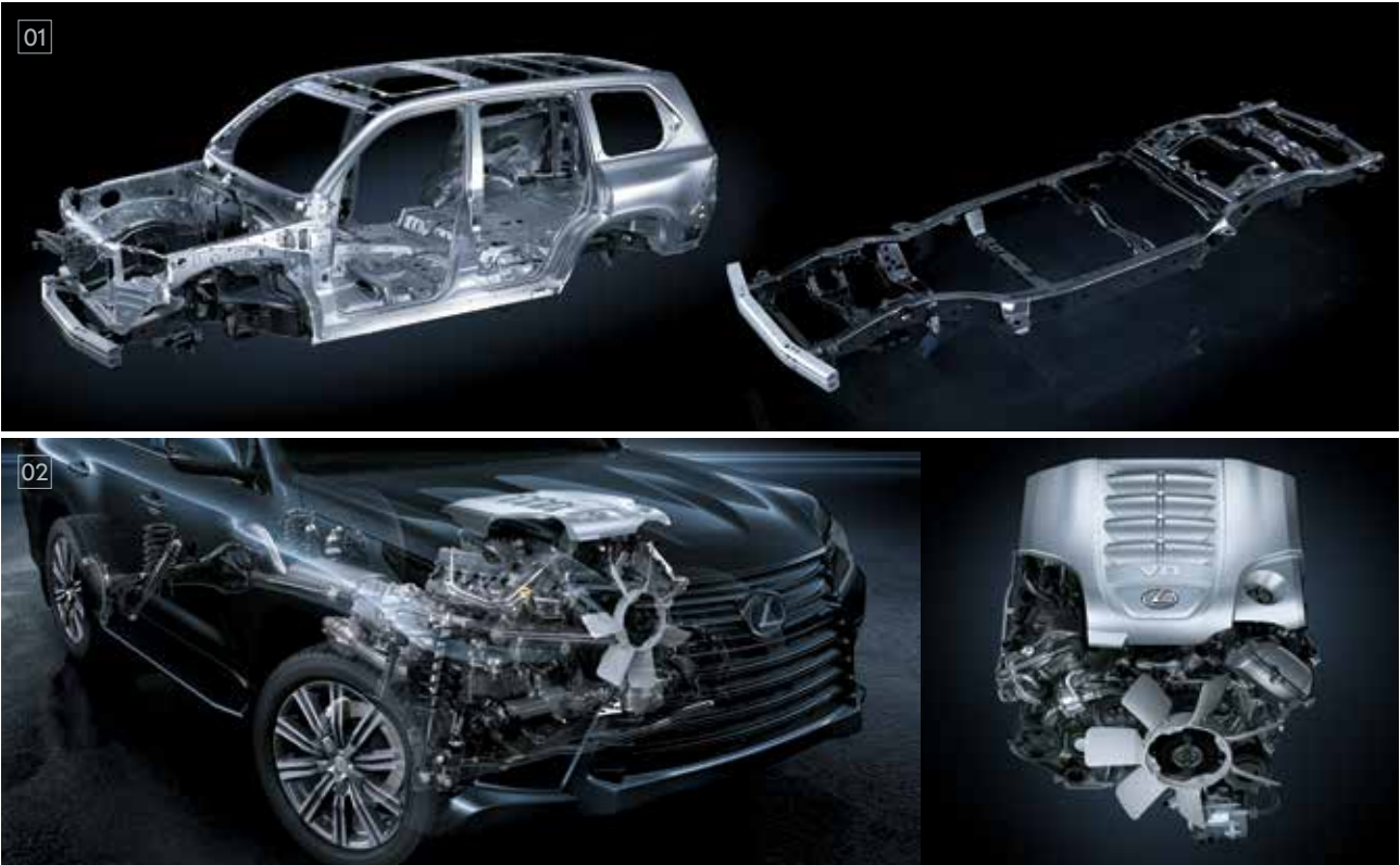
01/ Chassis The immense strength and outstanding rigidity essential to peerless off-road performance are the products of an exceptionally strong frame made with extensive use of high-tensile steel. In addition to outstanding off-road performance, it helps make the LX a robust and safe vehicle.
