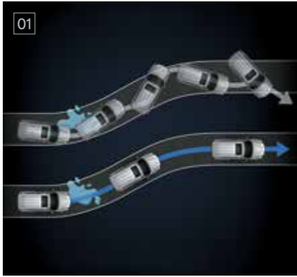
01 / A-TRC (Active Traction Control System) A-TRC helps enhance the ability to grip the road, especially when starting off or accelerating on uneven or slippery surfaces. Corrective measures are applied the moment the risk of wheelspin is detected, to help maintain traction.
