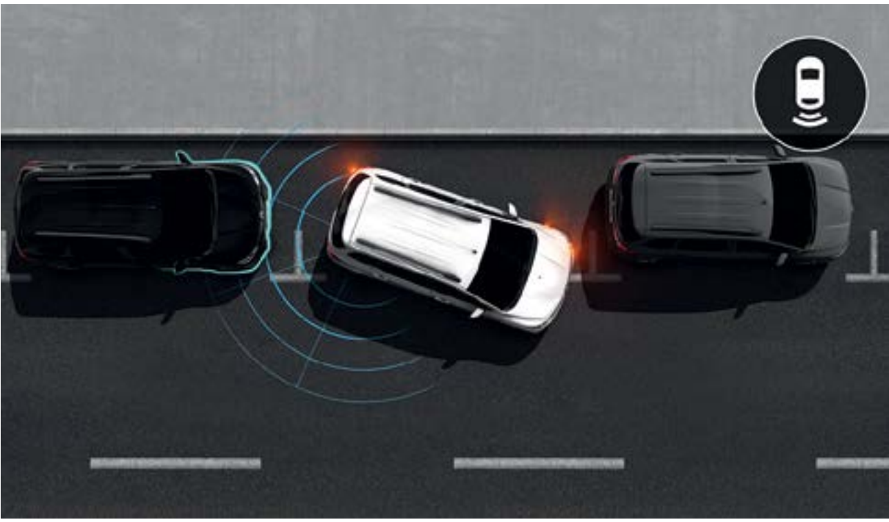
reverse parking sensor with camera Ultrasonic sensors in the rear bumper measure the distance between the vehicle and an obstacle.
